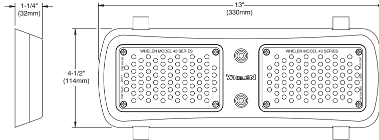
Model FLKIT optional foam rubber shroud for windshield mounting.
